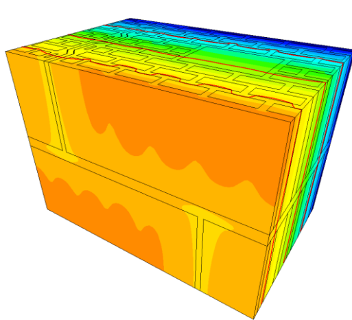
Figure 7. Example 2 isotherms
