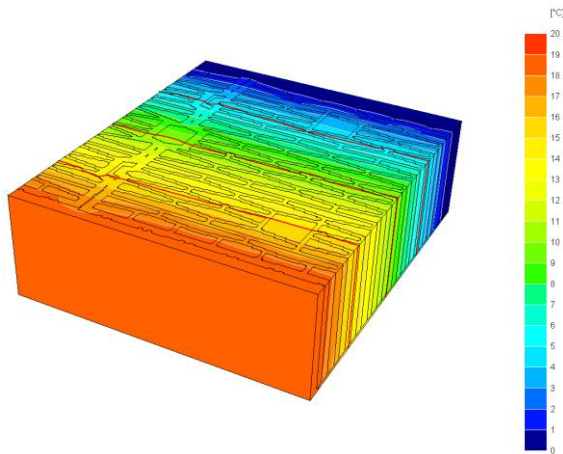
Figure 13. Example 3 isotherms
