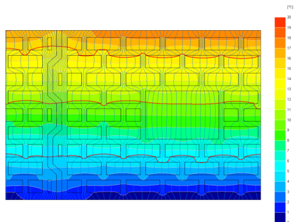
Figure 4. Results obtained by BISCO
