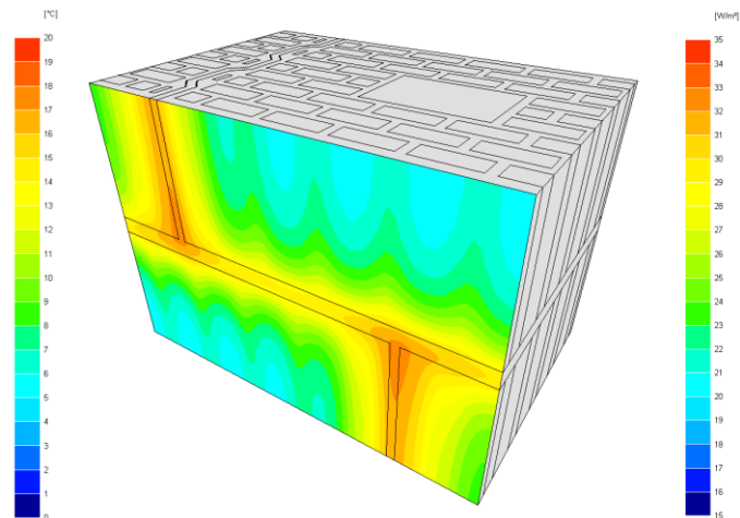
Figure 8. Example 2 heat flow densities
