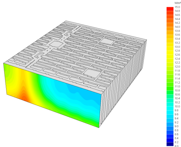
Figure 14. Example 3 heat flow densities
